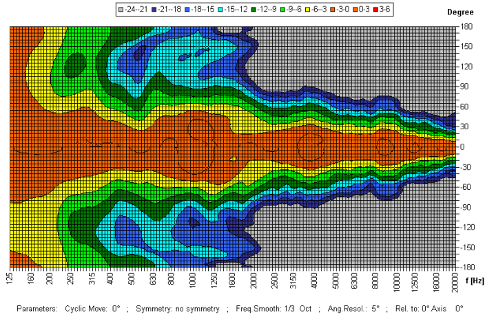
Side View Ver. Polarplots 500 Hz Octave 6 dB/div
