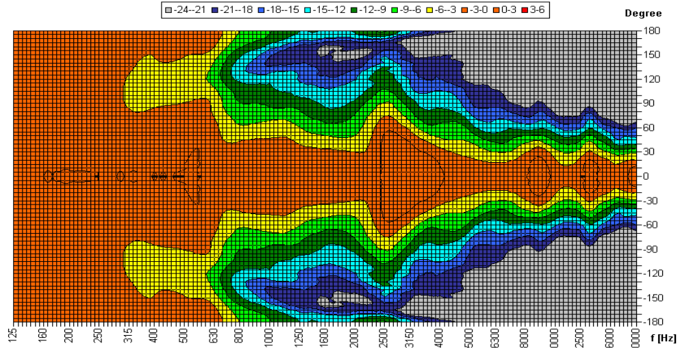
Top View Hor. Polarplots 500 Hz Octave 6 dB/div
