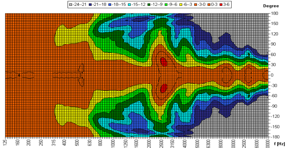
Side View Ver. Polarplots 500 Hz Octave 6 dB/div
